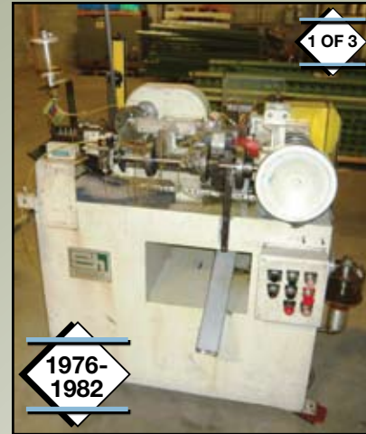
Sleeper & Hartley Mdl. 4116 Four-Slide
